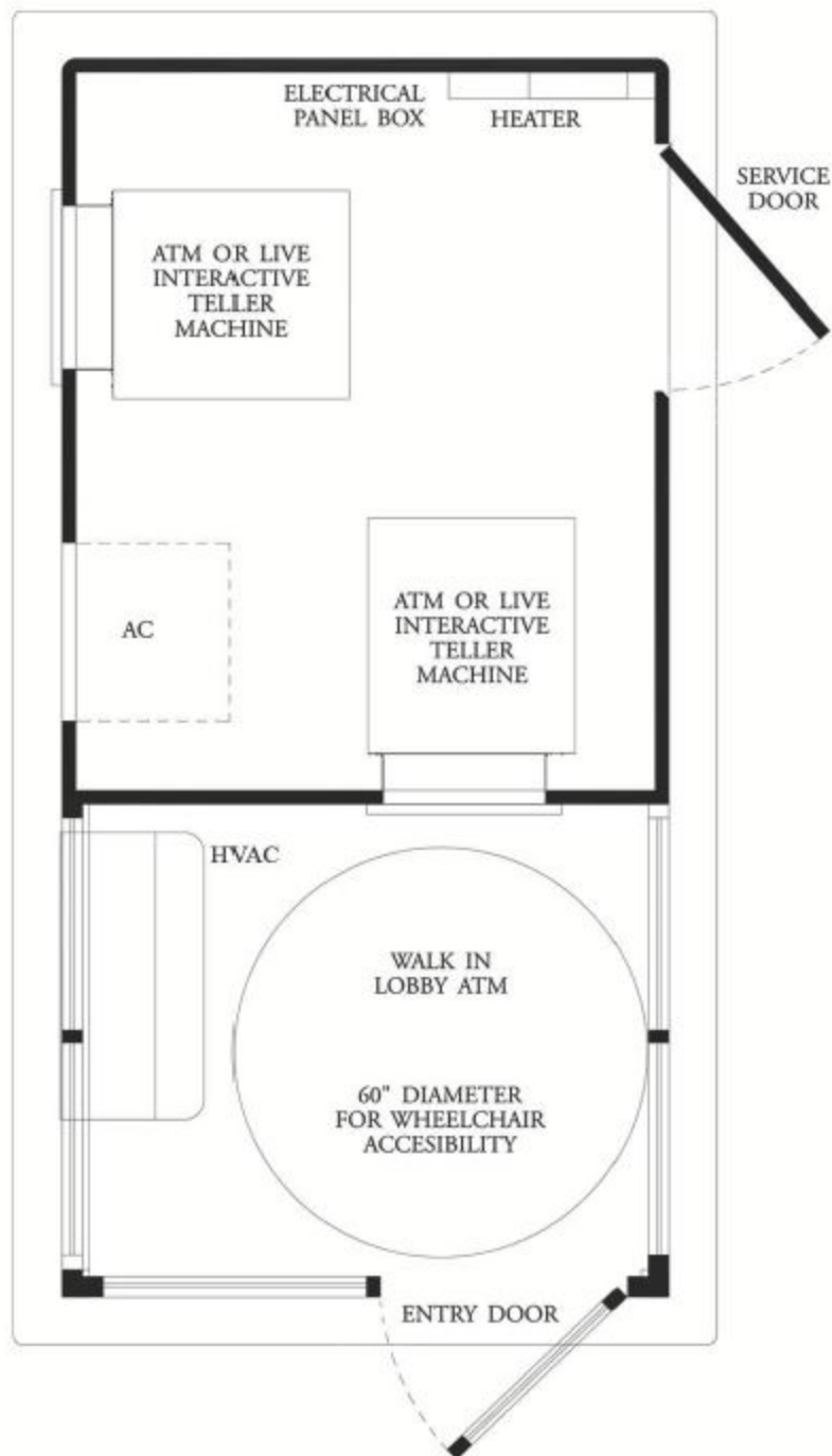
HERITAGE ELECTRONIC MINI-BRANCH SET-UP FOR WALK-IN LOBBY ATM, EXTERIOR WALK-UP OR DRIVE-UP ATM (SHOWN WITH OPTIONAL CANOPY)
